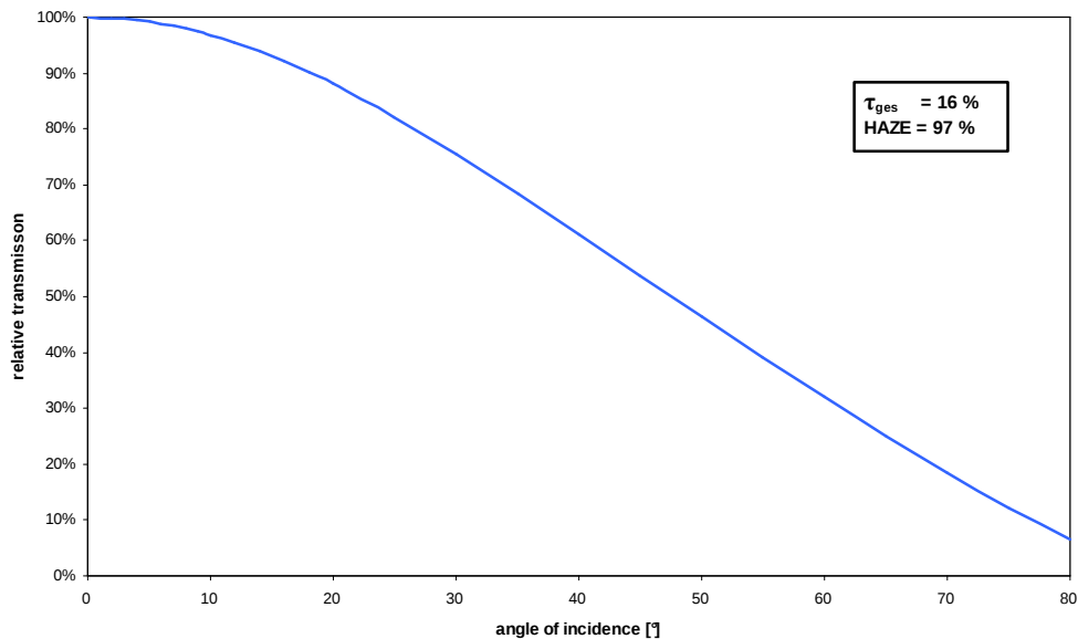
decrement of transmission in relation to incidence (wall thickness 1 mm)
